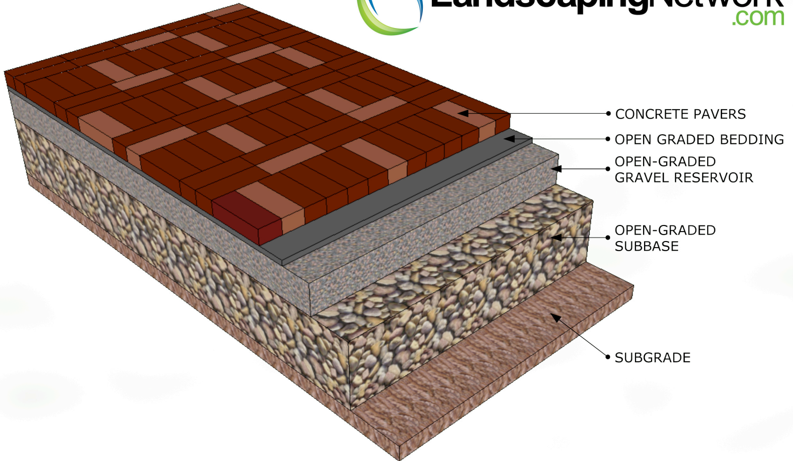
CROSS SECTION OF PAVER INSTALLATION
